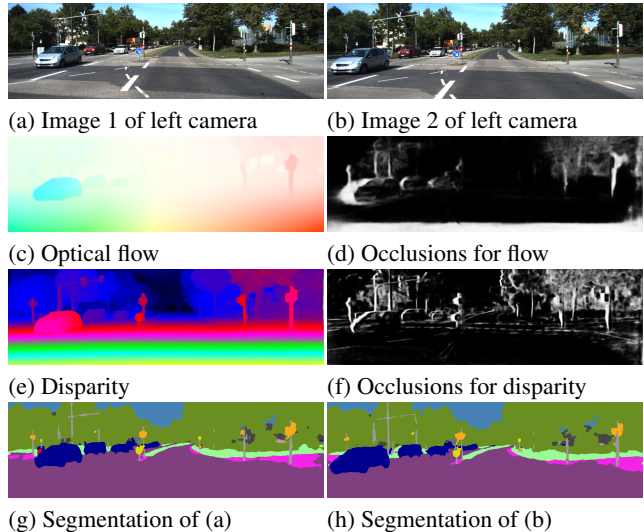
Figure 1. Given stereo videos, we train compact networks for several holistic scene understanding problems by sharing features.
