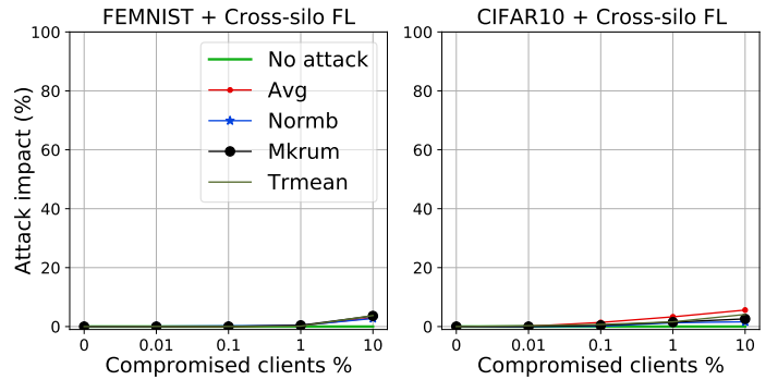
Figure 8: All data poisoning attacks have negligible impacts on cross-silo FL, when compromised clients are concentrated in a few silos or distributed uniformly across silos (Section V-D).
