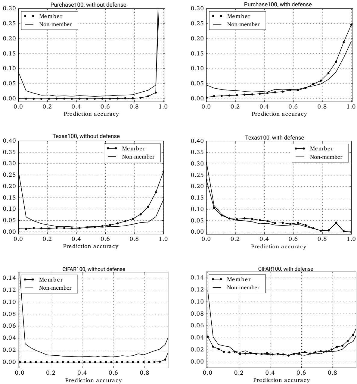
Figure 7: Distribution of the classifier’s prediction accuracy on members of its training set versus non-member data samples.
