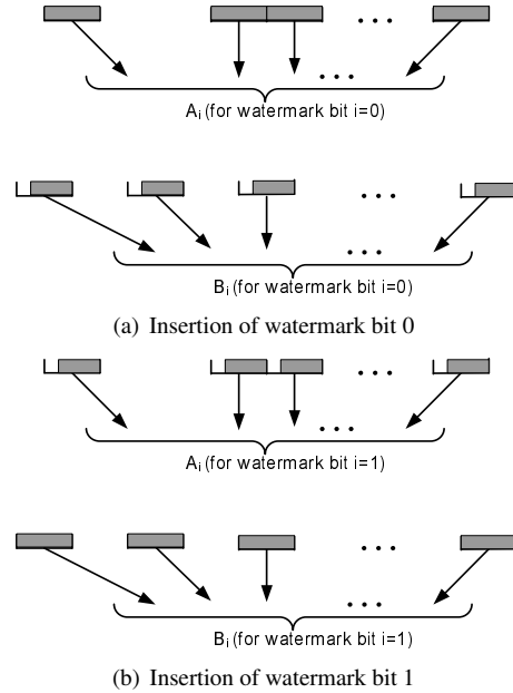
Figure 6: ICBW bit insertion
