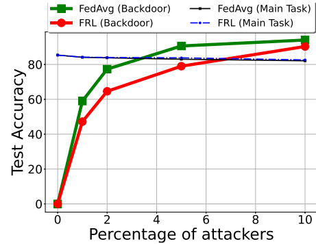
(b) Edge-Case backdoor results
