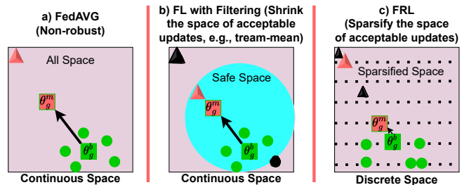
Figure 1: The space of client updates. Green circles represent benign updates and red triangles represent malicious updates. To defend against poisoning, existing robust AGRs filter the updates by creating a safe space (continuous \in \mathbb{R}^d ). On the other hand, FRL limits the choices of clients by enforcing a discrete space of updates (a permutation of integers \in [1, d] ). \theta_g^b (green square) demonstrates the aggregated model for benign users, and \theta_g^m (red square) demonstrates the aggregated model considering malicious updates. Black objects are updates that are ruled out by the server.
