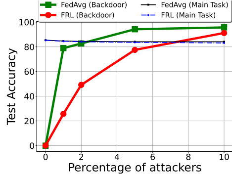
(a) Semantic backdoor results
