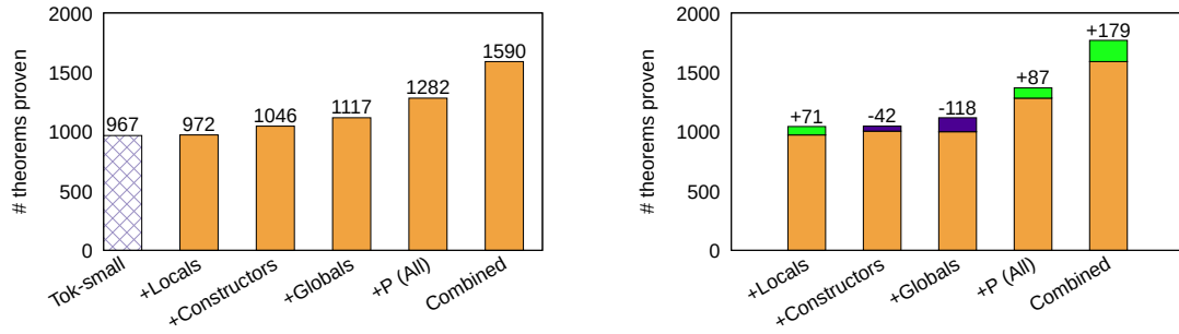
(a) The impact of category vocabulary indexing on three identifier categories (without subwords or paths): local variables, type constructors, and global definitions.
