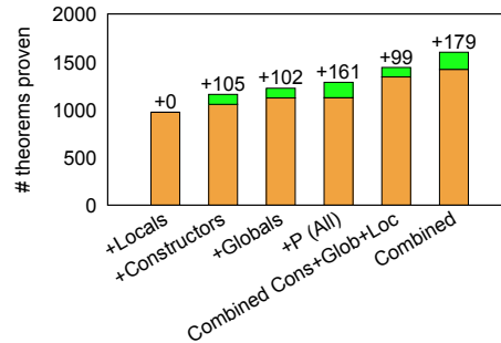
(c) The impact of fully-qualified path encoding of type constructors and global definitions (with category vocabulary indexing but without subwords).
