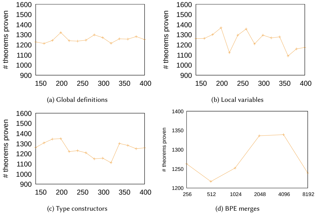
Fig. 8. The impact of different vocabulary thresholds for the various categories of identifiers. A smaller threshold means the vocabulary is larger.
