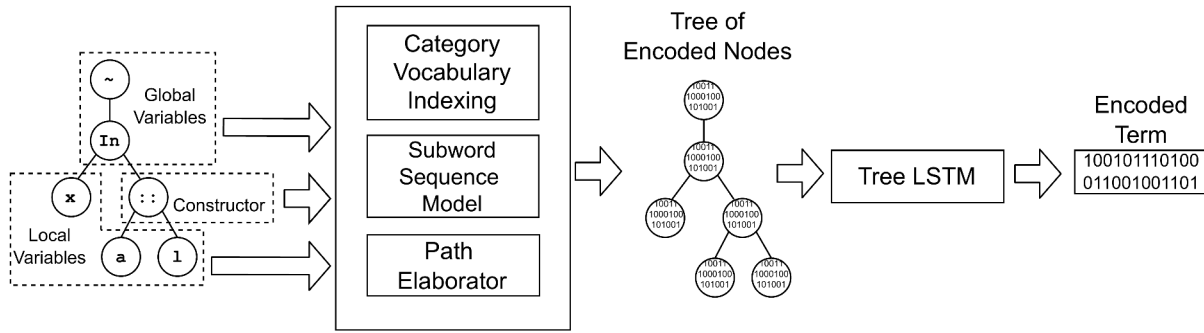
Fig. 4. The architecture of Passport’s identifier processing.
