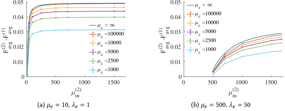
Fig. 6. Average gate fidelity differences in two entanglement request arrival and generation rate regimes. For all simulations, T_1^{(1)} = T_1^{(2)} = 0.00286\text{s} and T_2^{(1)} = T_2^{(2)} = 0.001\text{s} ; \mu_m^{(1)} = 1667\text{Hz} , \lambda_c = 150 and \lambda_m = 1000 .
