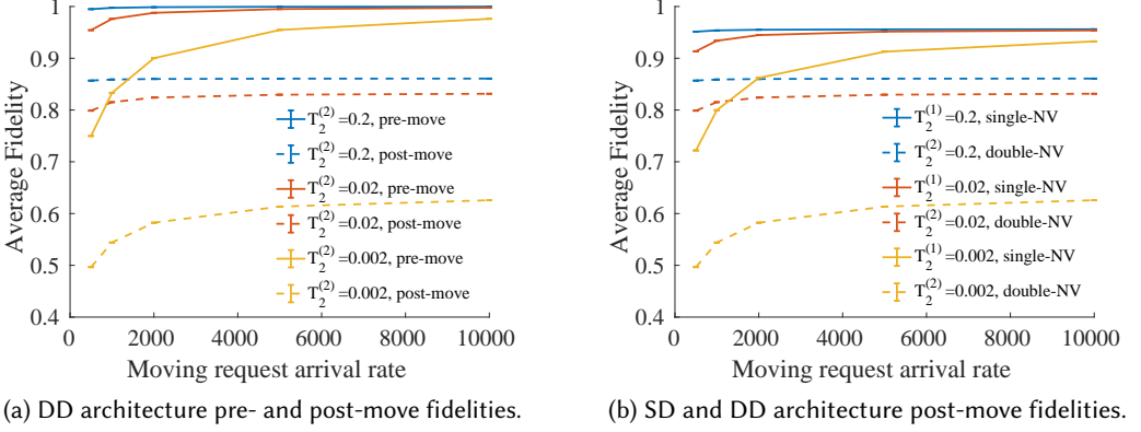
Fig. 10. Pre- and post-move fidelities for the DD architecture, (a), and post-move fidelities for the two architectures, (b). Here, T_1^{(1/2)} = 2s , \lambda_e = 1 , \mu_e = 10 , \lambda_c = 150 , \mu_c = 10^5 , \mu_m^{(1)} = 1667\text{Hz} , and \mu_m^{(2)} = 700\text{Hz} .
