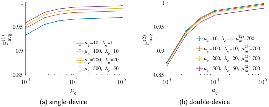
Fig. 15. Average gate fidelities for computational jobs for the SD architecture, (a), and the DD architecture, (b). Here, T_1^{(1)} = 10\text{s} , T_2^{(1)} = 0.01\text{s} , T_1^{(2)} = 2\text{s} , and T_2^{(2)} = 0.002\text{s} ; \mu_m^{(1)} = 1667\text{Hz} for all SD simulations. For all experiments, \lambda_c = 150 and \lambda_m = 1000 .
