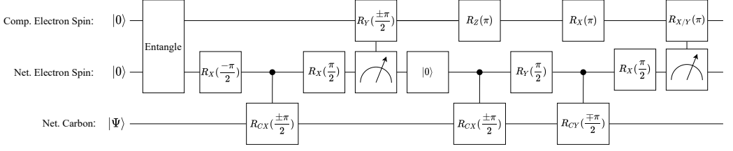
Fig. 13. Quantum circuit for moving a quantum state from the networking device electron spin into the computing device electron spin.
