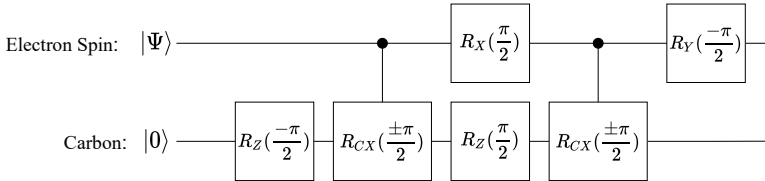
Fig. 12. Quantum circuit for moving a quantum state from the NV into carbon storage. Each gate applies noise onto the qubits it interacts with.
