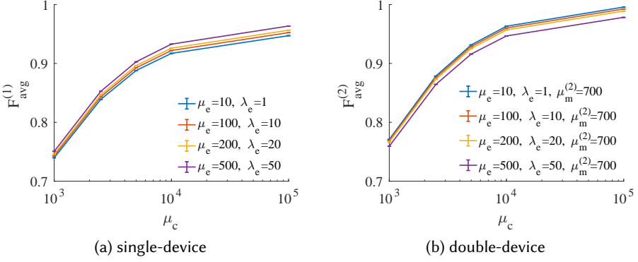
Fig. 14. Average gate fidelities for computational jobs for the SD architecture, (a), and the DD architecture, (b). Here, T_1^{(1)} = T_1^{(2)} = 0.00286\text{s} and T_2^{(1)} = T_2^{(2)} = 0.001\text{s} ; \mu_m^{(1)} = 1667\text{Hz} for all SD simulations. For all experiments, \lambda_c = 150 and \lambda_m = 1000 .
