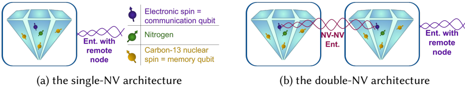
Fig. 2. An example of SD and DD architectures based on Nitrogen-Vacancy centers in diamond. Here, the electron spin (purple) acts as an optical interface that can be used as a networking or computing component. Nitrogen (green) and the Carbon-13 spins (yellow) in the surrounding diamond material can be used as computing components. See Appendix D for further details about this platform.
