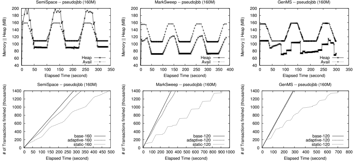
Figure 8: Dynamic Memory Allocation (pseudojbb): Heap Adjustment and Throughput
