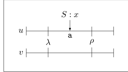
Figure 9: A letter occurs between rankers r, r' in u but not in v
