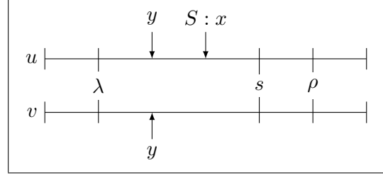
Figure 7: x and y are in the same section
