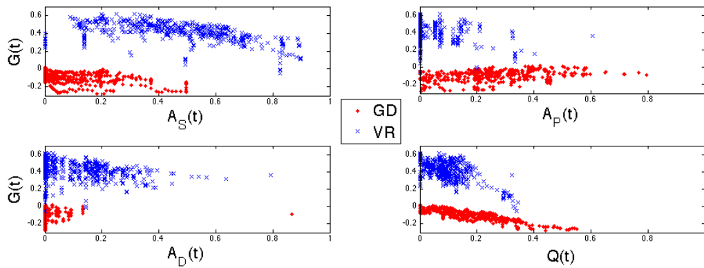
Fig. 4: The external processes A_S(t) , A_P(t) , A_D(t) , and Q(t) plotted against G(t) for GD (red dots) and VR (blue cross).
